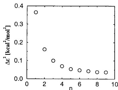
FIGURE 7 Dependence of \Delta \epsilon^2 on the number of hairpins (circles).
