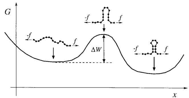
FIGURE 10 Sketch of the assumed pathway for the formation of a stem-loop structure in the presence of a stretching force f . A generalized reaction coordinate x is plotted along the horizontal axis and the free energy G along the vertical axis. The work that has to be exerted against the force to pull in the single strand needed for the formation of the stem-loop structure is denoted by \Delta W . In principle, the entropy difference between the random coil state on the left and the transition state also contributes to the barrier height; however, we assume that at typical stretching forces it is negligible compared to \Delta W .
