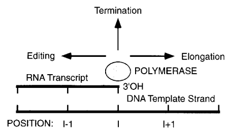
Fig. 1. Three competing pathways for the transcription complex at a given template position. The options are (i) to move forward along the template with the concomitant elongation of the RNA chain by one nucleotide residue, (ii) to move backward along the template (with or without shortening the transcript by one or more residues), or (iii) to dissociate from the template, resulting in release of the nascent RNA.
